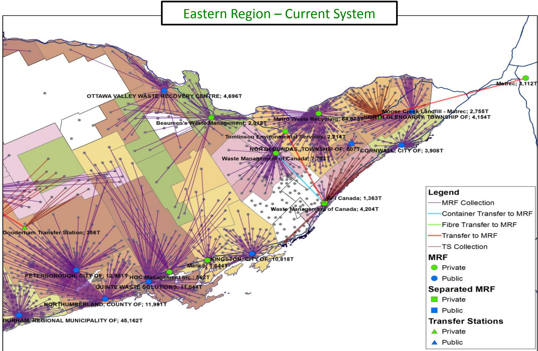
FIGURE 1: Current System Infrastructure and Material Flow for the Eastern Region
