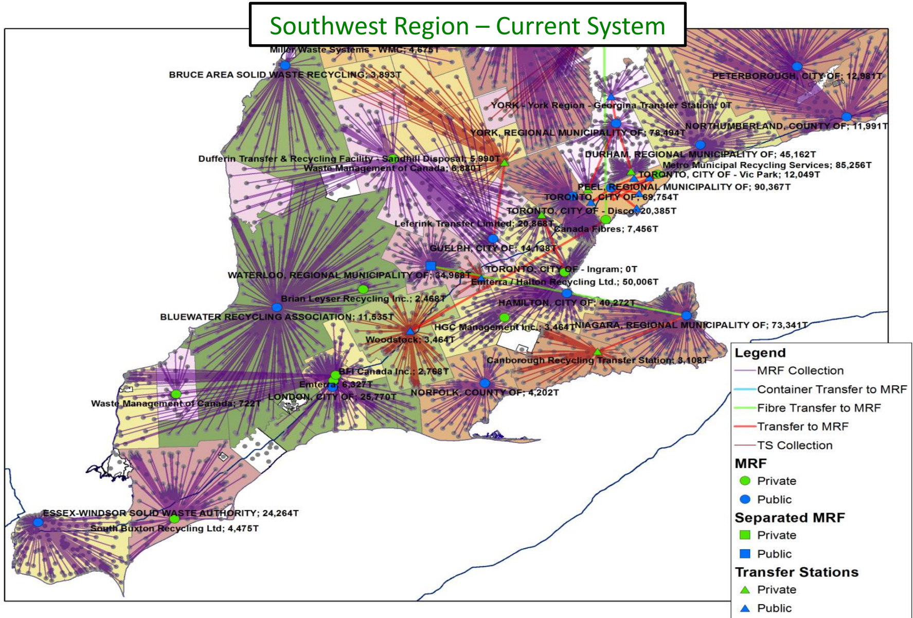
FIGURE 2: Current System Infrastructure and Material Flow for the Southwestern Region
